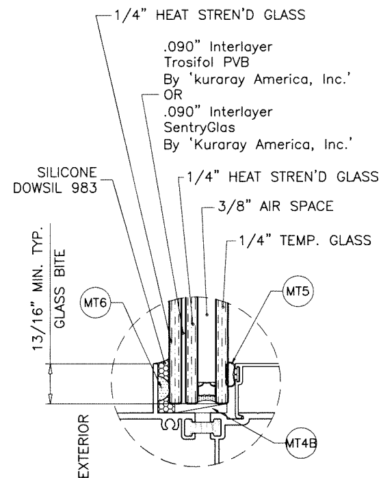
GLASS TYPE 'E' 1-1/4" OVERALL LAM. INSUL. GLASS
