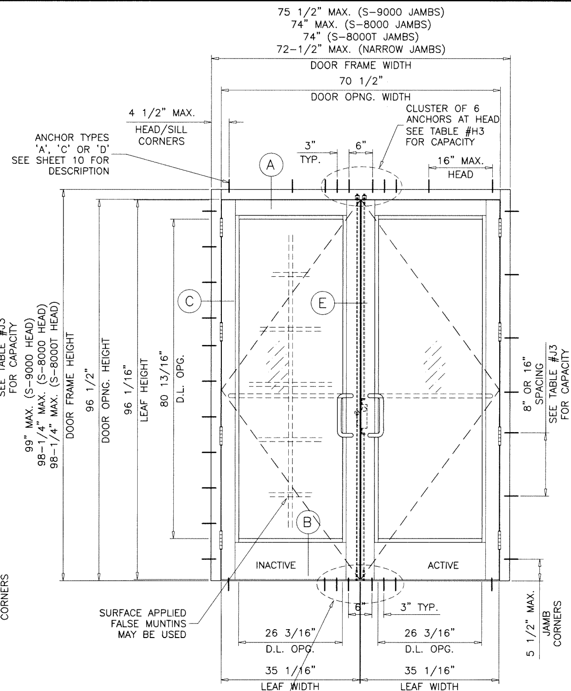
TYPICAL ELEVATION
