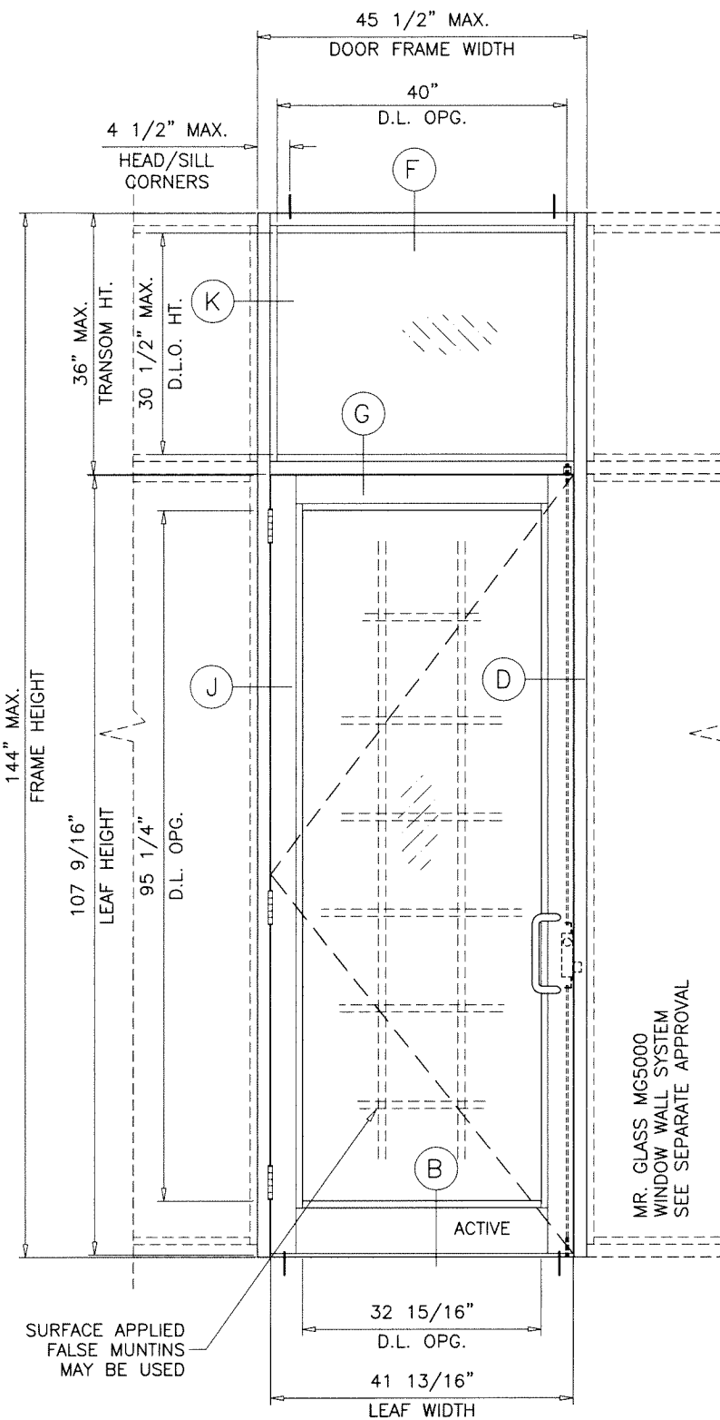
TYPICAL ELEVATION SINGLE (O/X) (ES-8000 TRANSOM)
