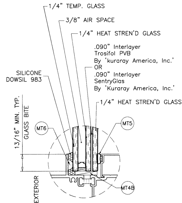
GLASS TYPE 'E-R' 1-1/4" OVERALL INSUL. LAM. GLASS
